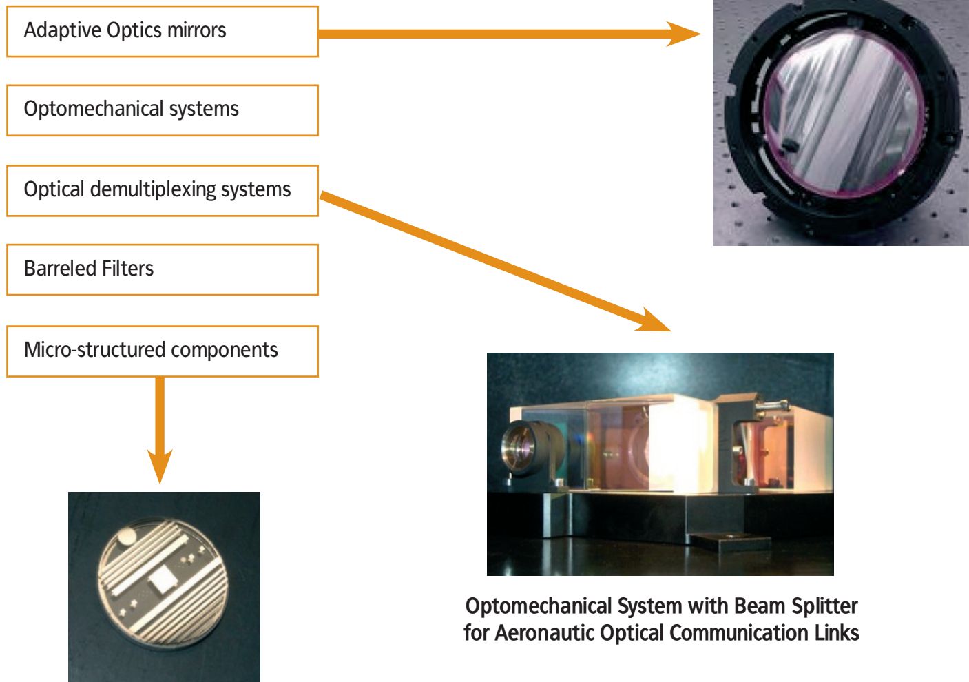
Micro-structured Component Lithography & Etching using microelectronics technologies
