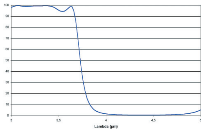
Transmittance measurement
