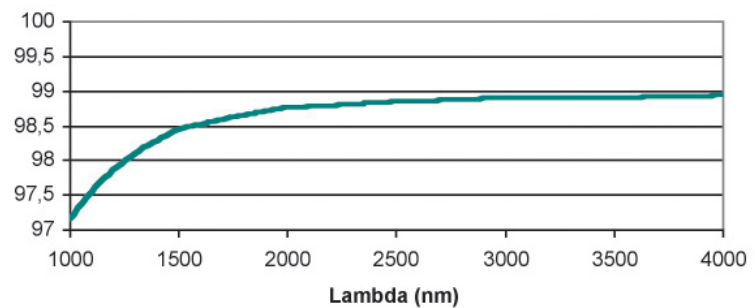
Gold-ZnS Reflectance Measurement
