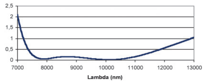
AR 8-12µm on ZnSe Reflectance Measurement
