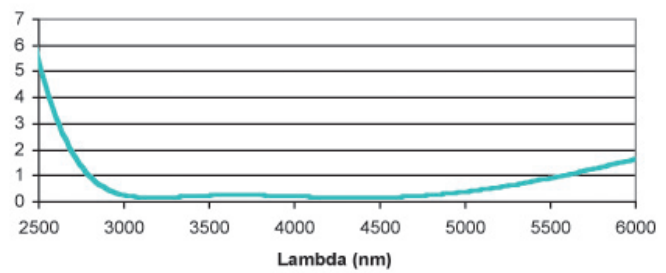
AR 3-5µm on Ge Reflectance Measurement
